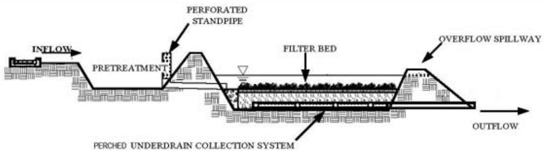
PROFILE
