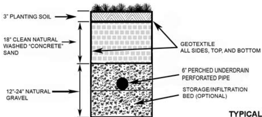
TYPICAL SECTION
