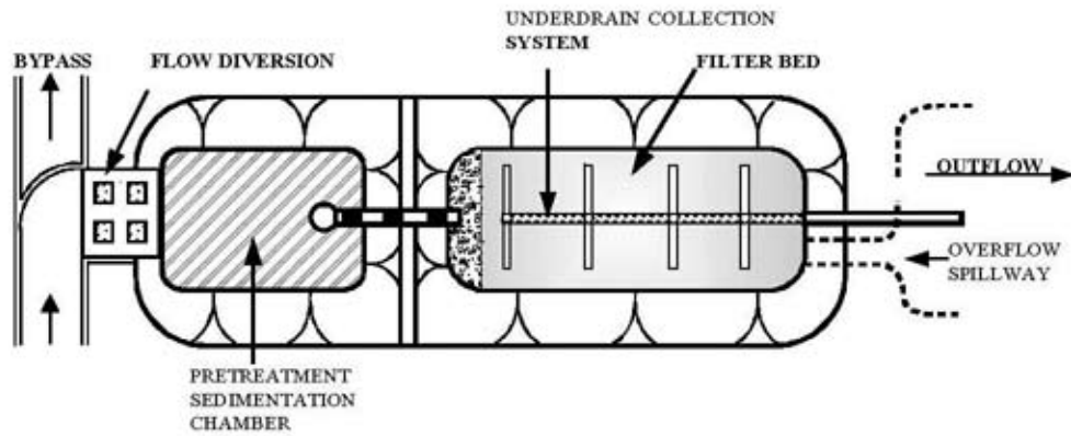
PLAN VIEW
